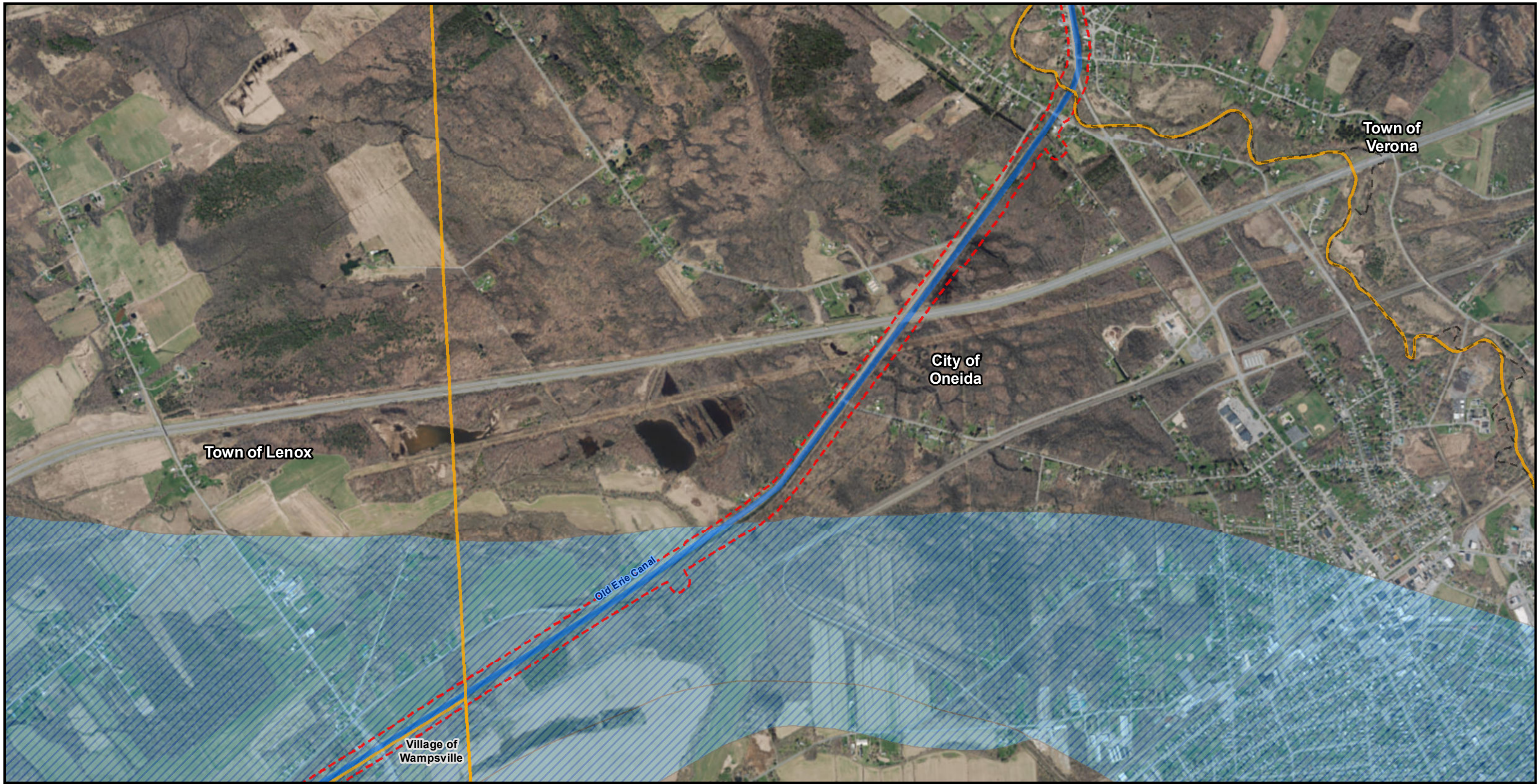
Figure 59F: Aquifers
